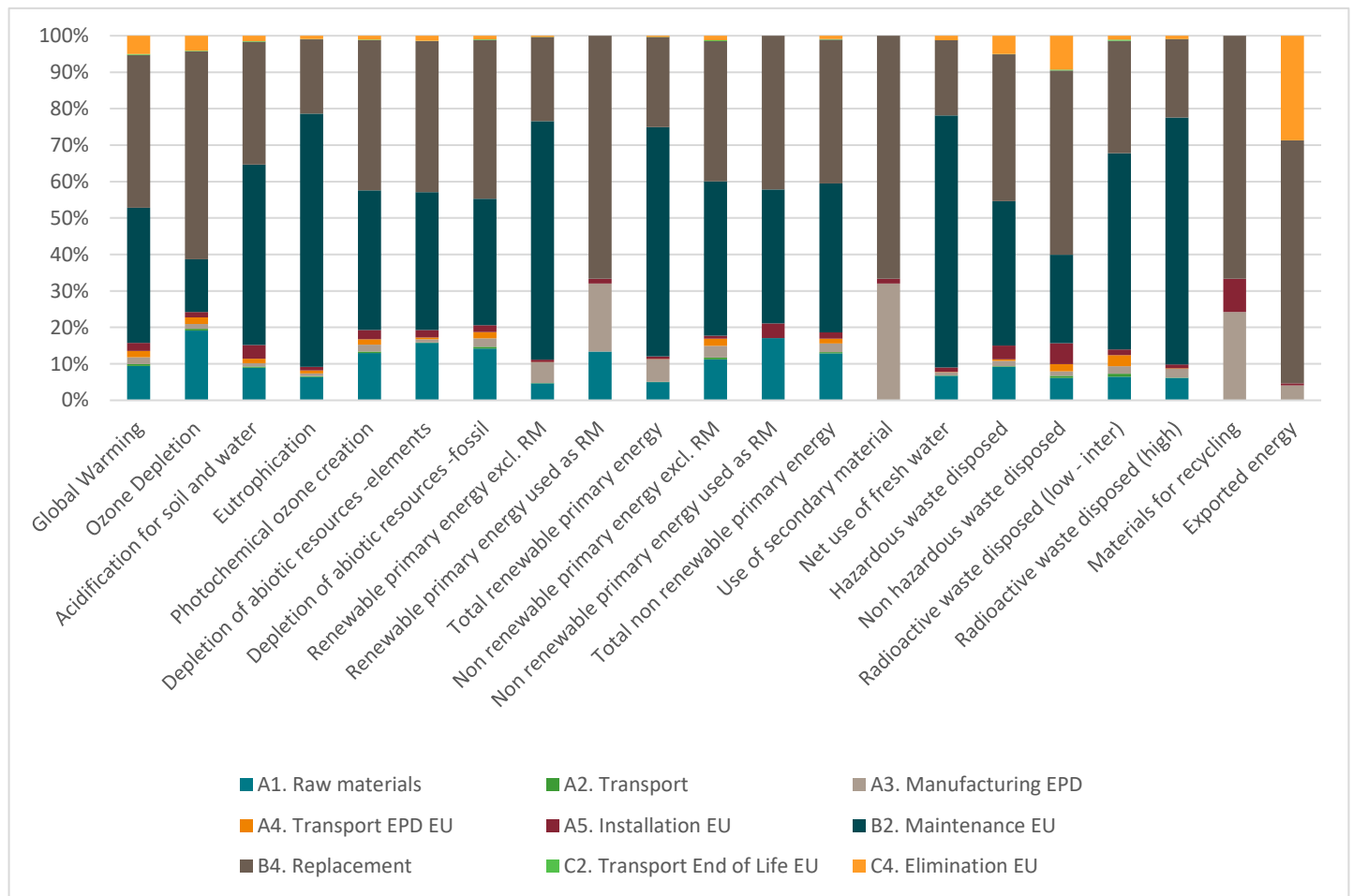
Figure 8: Graph depicting selection of impact indicator results calculated according to EN 15804 – Europe
