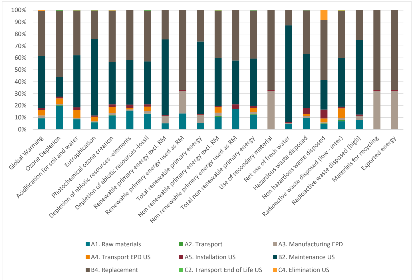
Figure 6: Graph depicting selection of impact indicator results calculated according to EN 15804 - US
