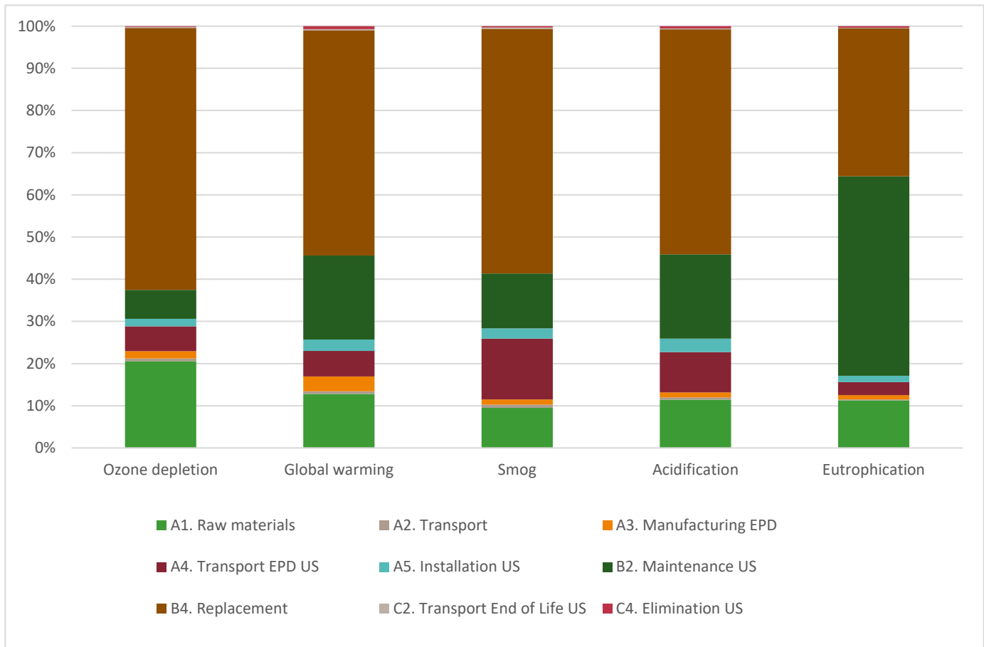
Figure 5: Graph depicting the impact indicators as calculated by the TRACI method
