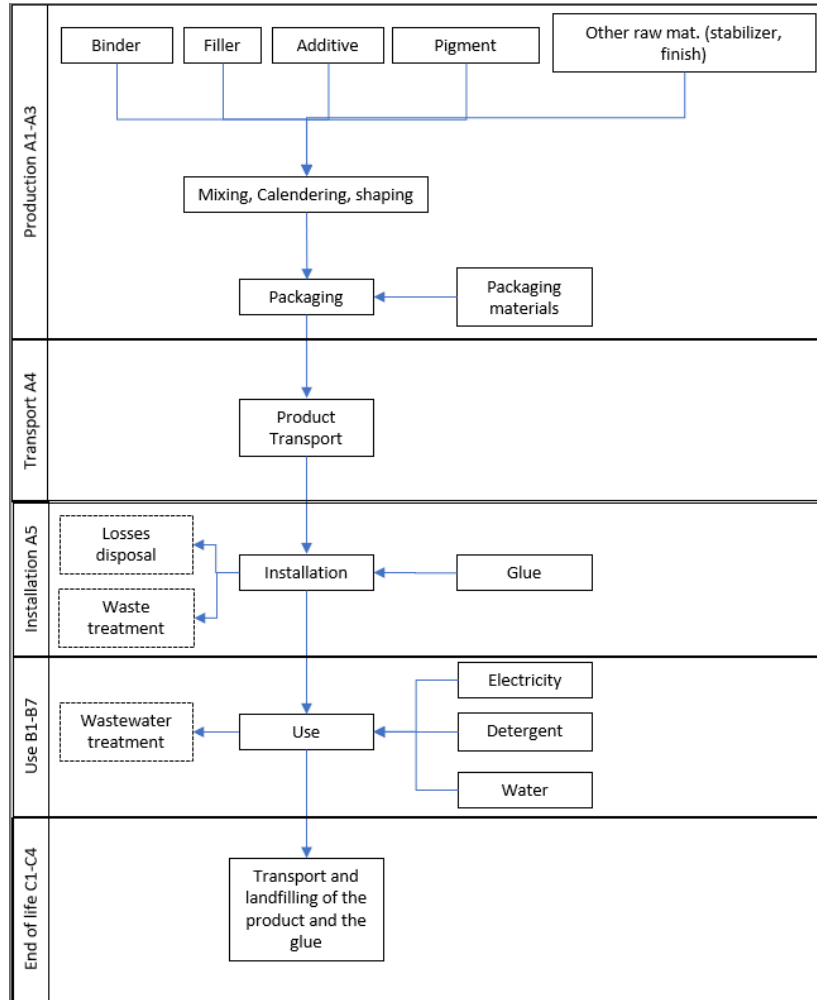
Figure 3: Flow product diagram
