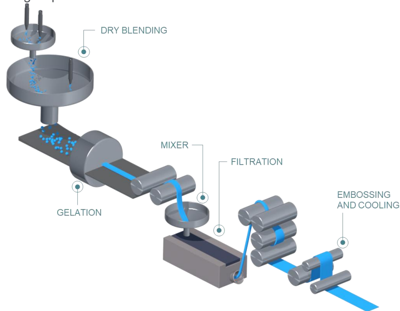
Figure 4: Manufacturing flow diagram
